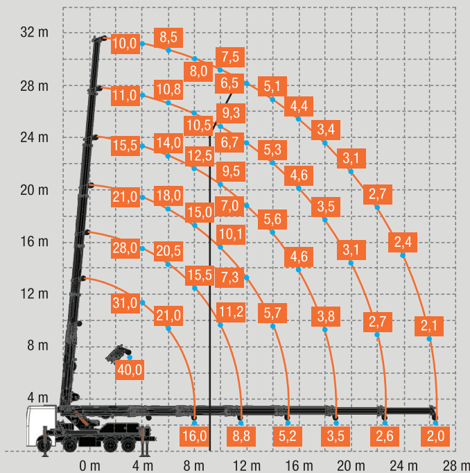
T4000 + Jib
